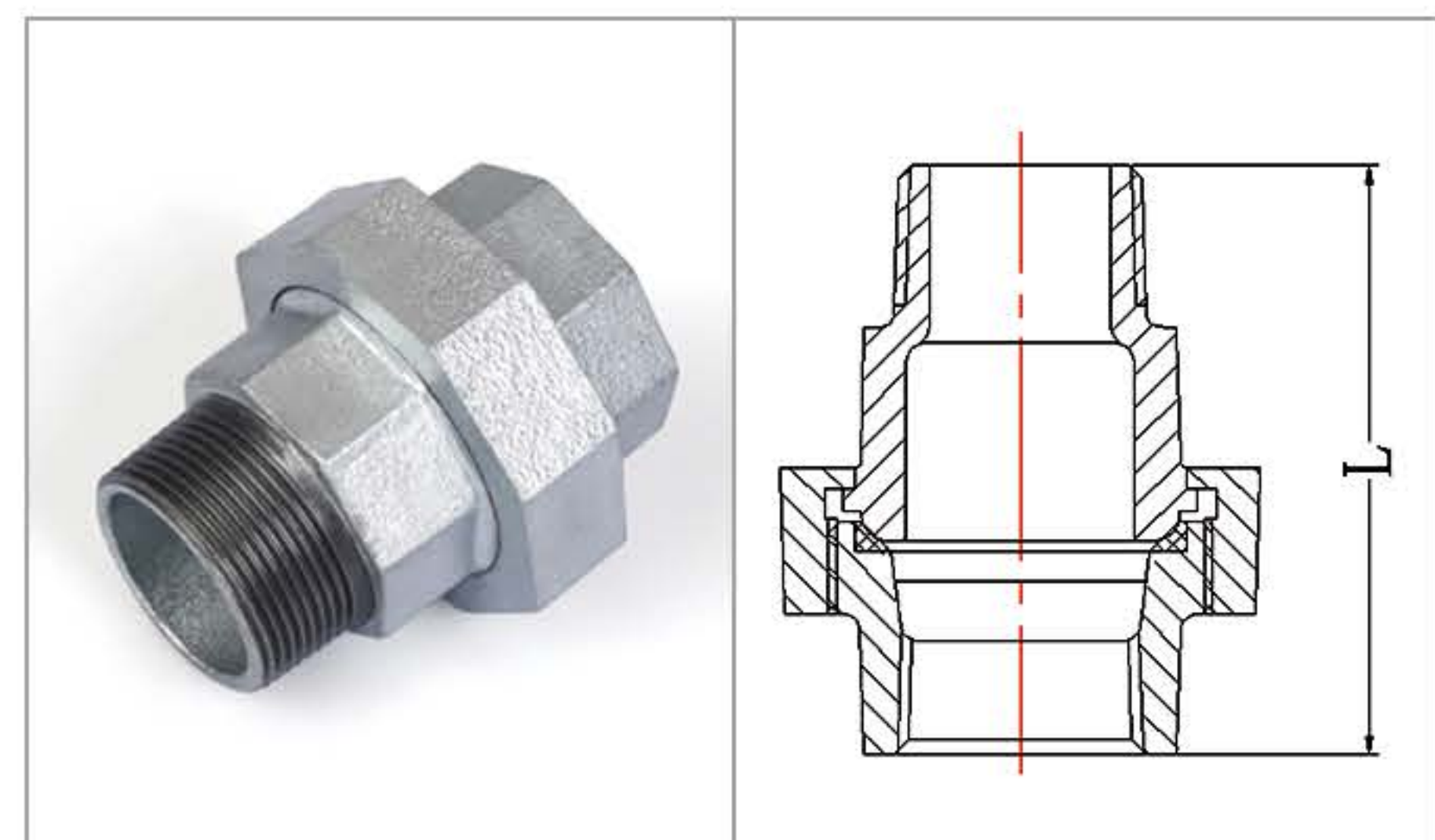
Fig.343 Brass Unions, Taper Seat, M&F
