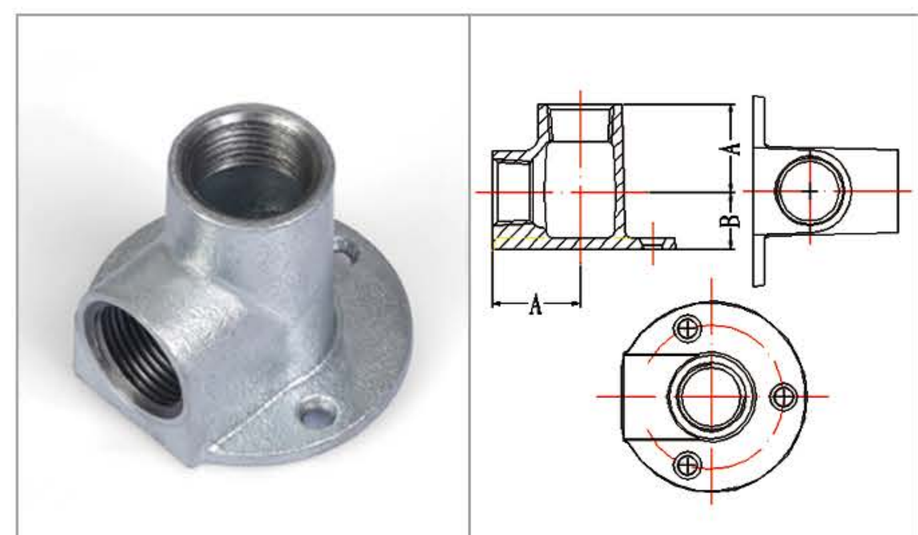
Fig.1221 Banded Side Outlet Elbow
