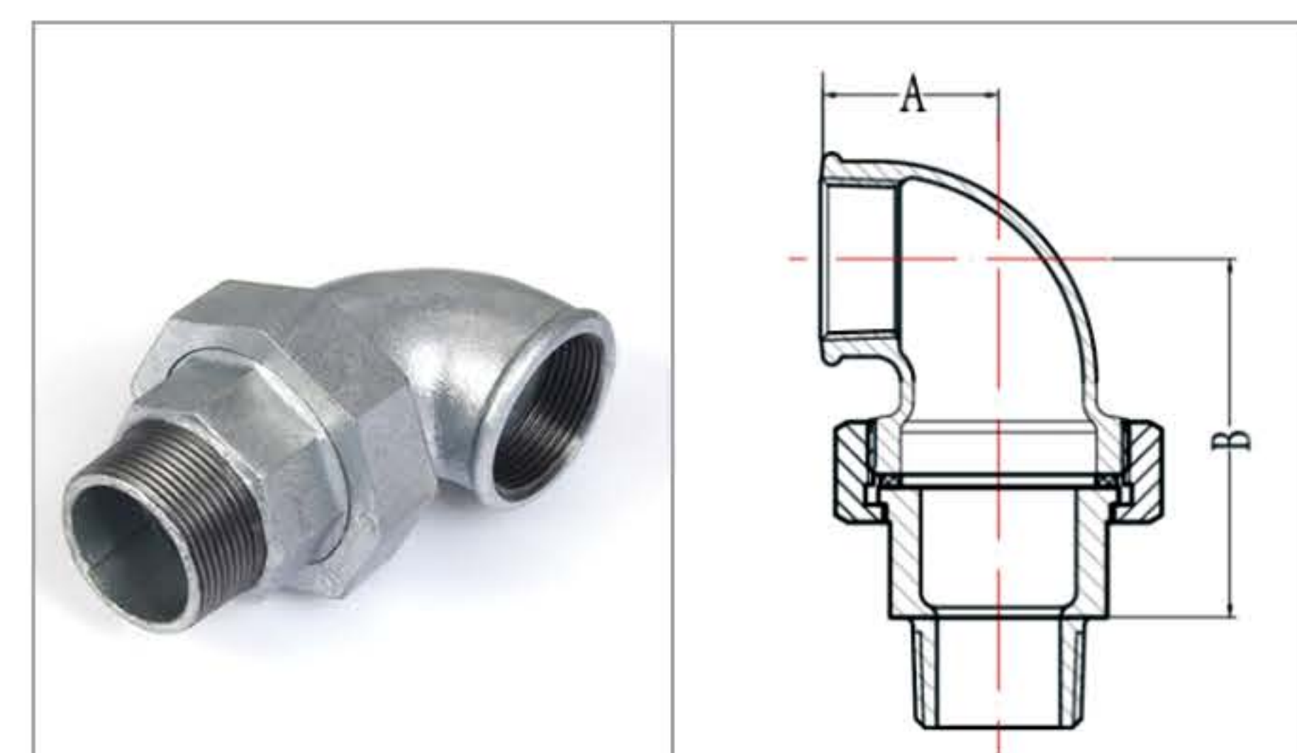
Fig.98 M&F Conical Union Elbow
